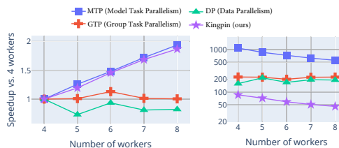
Figure 10: Worker scalability test.
